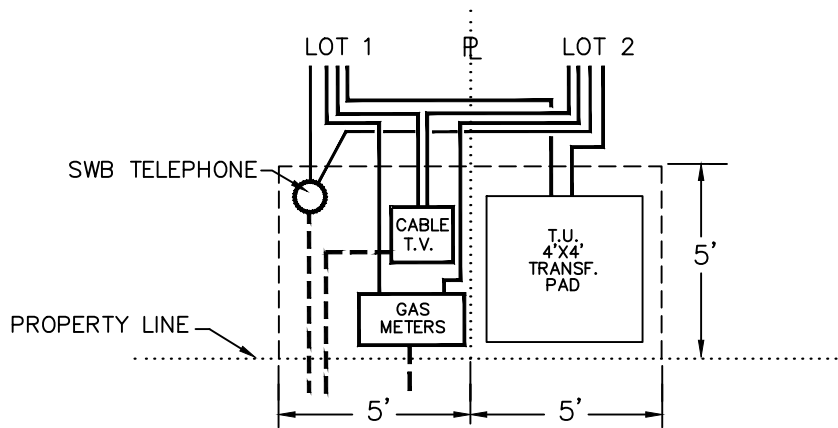
TYPICAL 5' X 10' UTILITY INSET FOR RESIDENTIAL SERVICE
